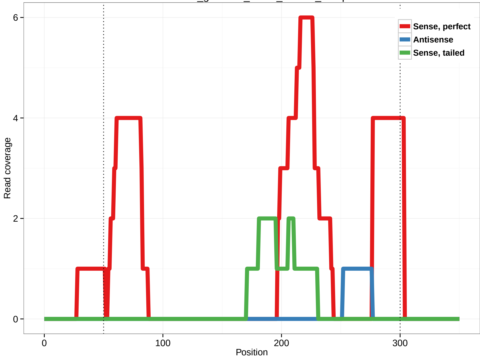
rheMac3_genscan_chr14_119.69_15.5p
