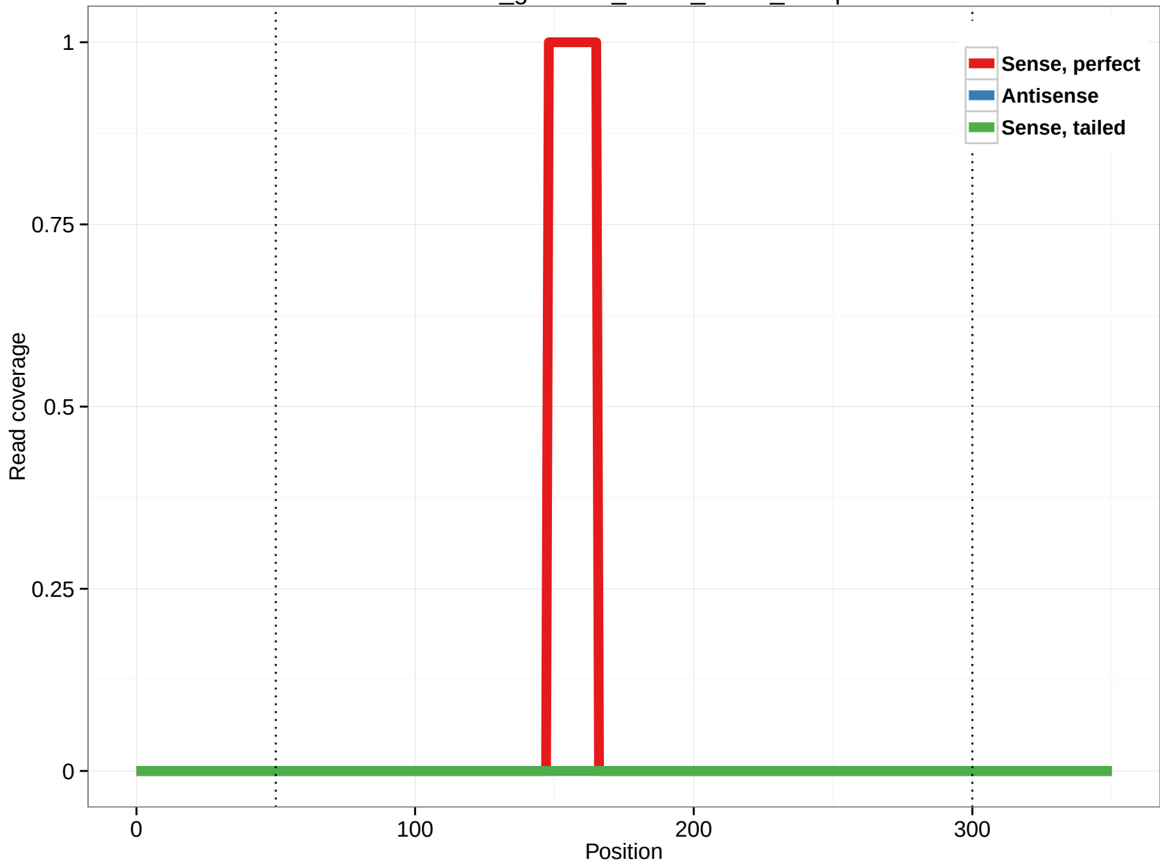
rheMac3_genscan_chr14_119.4_21.3p
