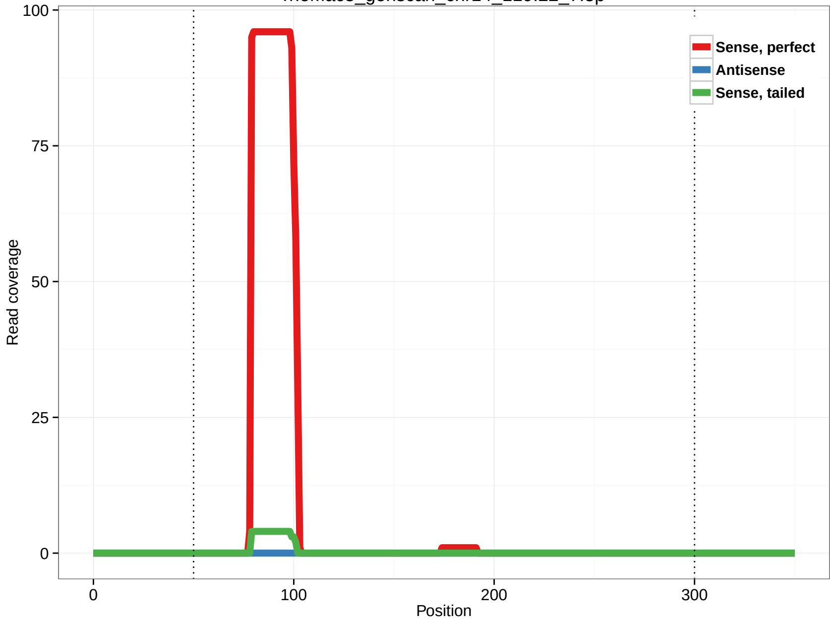
rheMac3_genscan_chr14_119.22_7.3p
