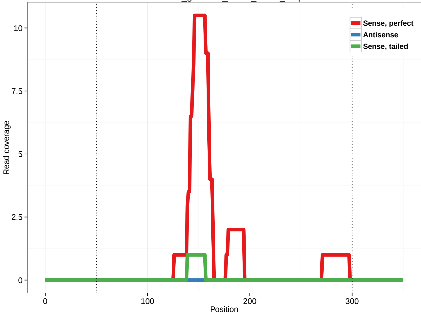
rheMac3_genscan_chr14_118.6_1.3p
