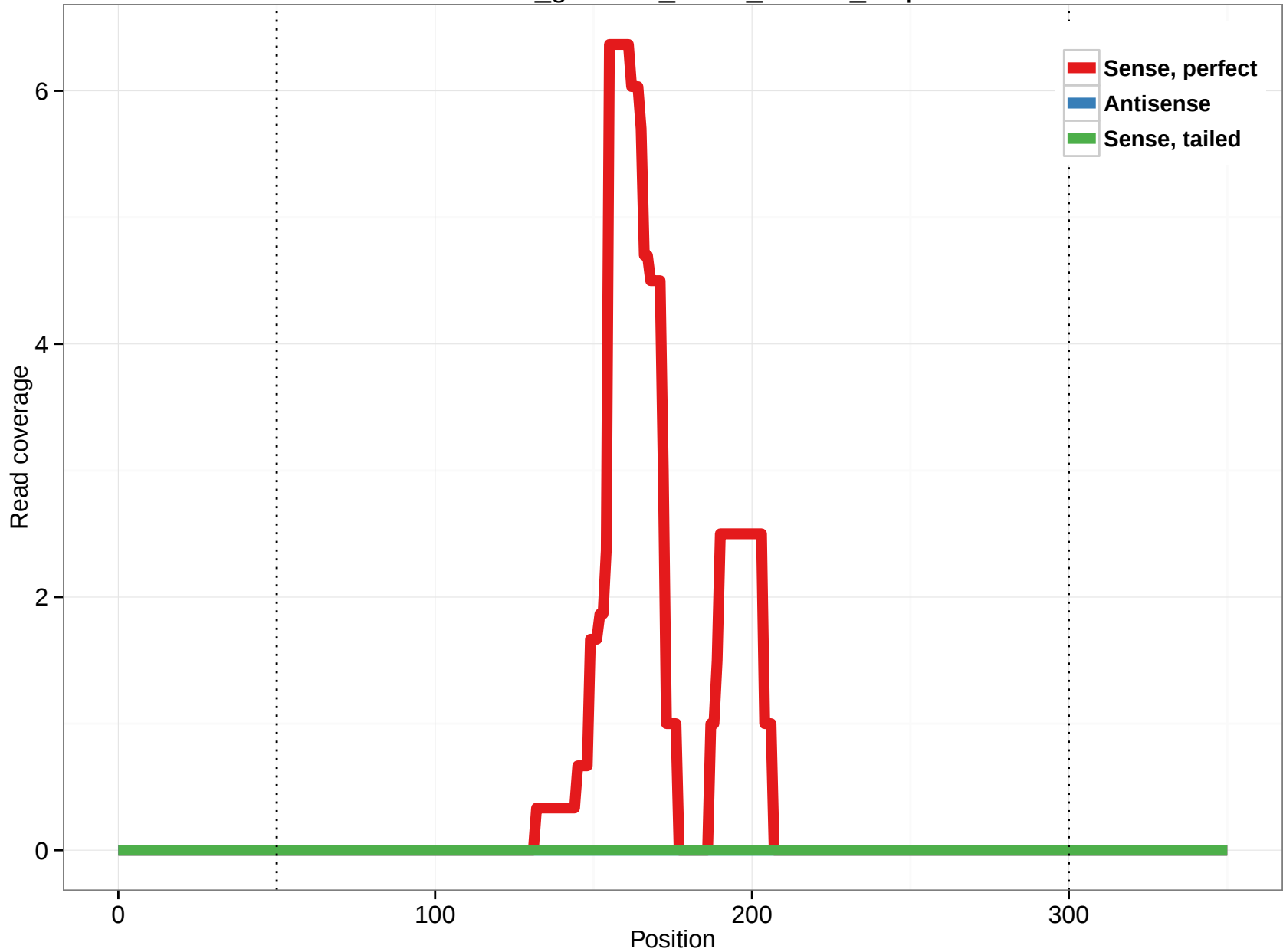
rheMac3_genscan_chr14_116.15_0.3p
