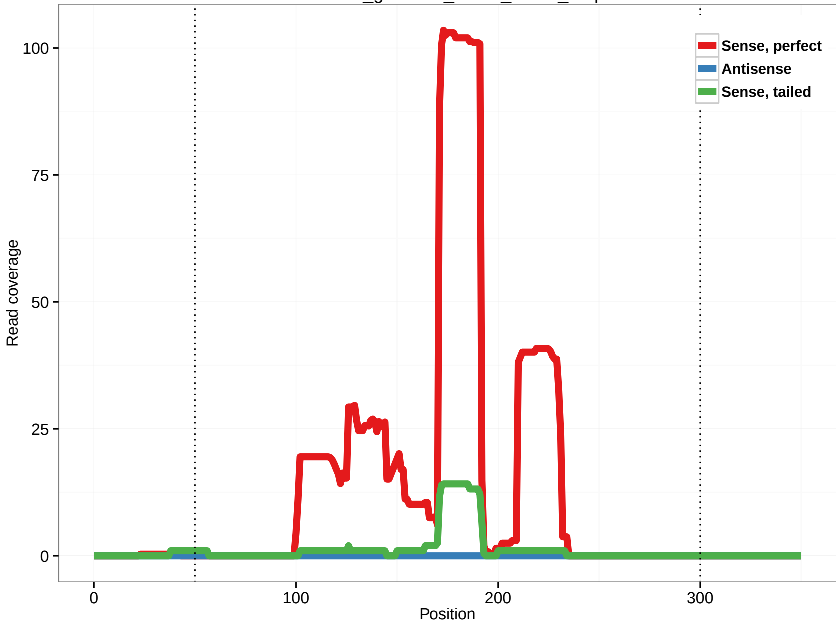
rheMac3_genscan_chr14_106.7_2.3p
