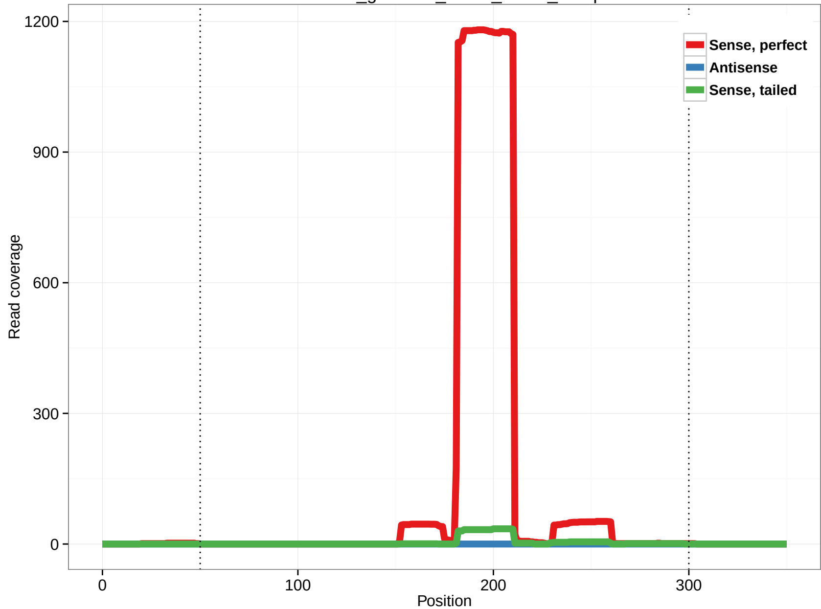
rheMac3_genscan_chr14_106.6_14.5p
