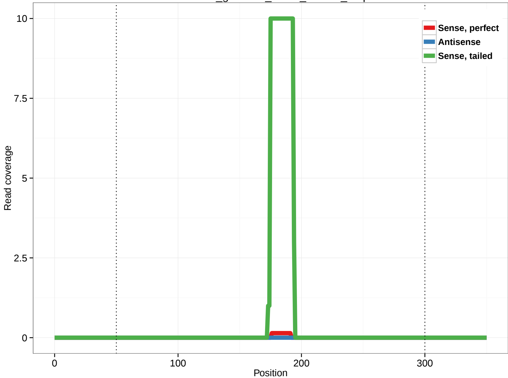
rheMac3_genscan_chr14_106.35_2.3p
