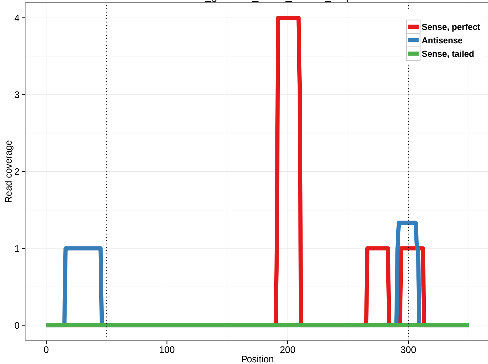
rheMac3_genscan_chr14_106.17_4.5p
