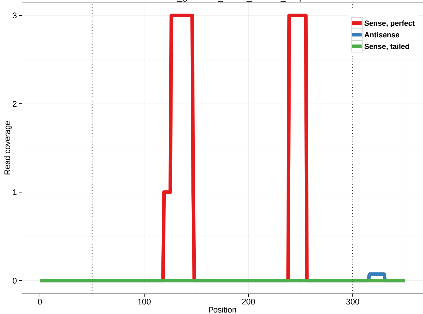
rheMac3_genscan_chr14_104.38_3.5p
