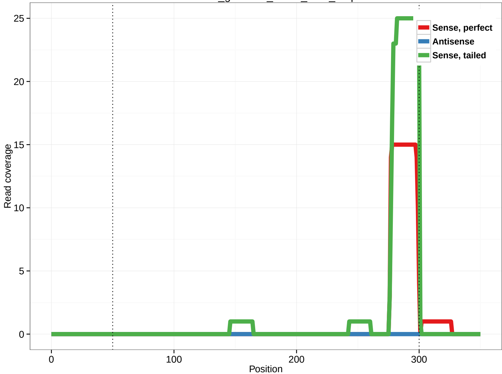
rheMac3_genscan_chr14_06.9_2.3p
