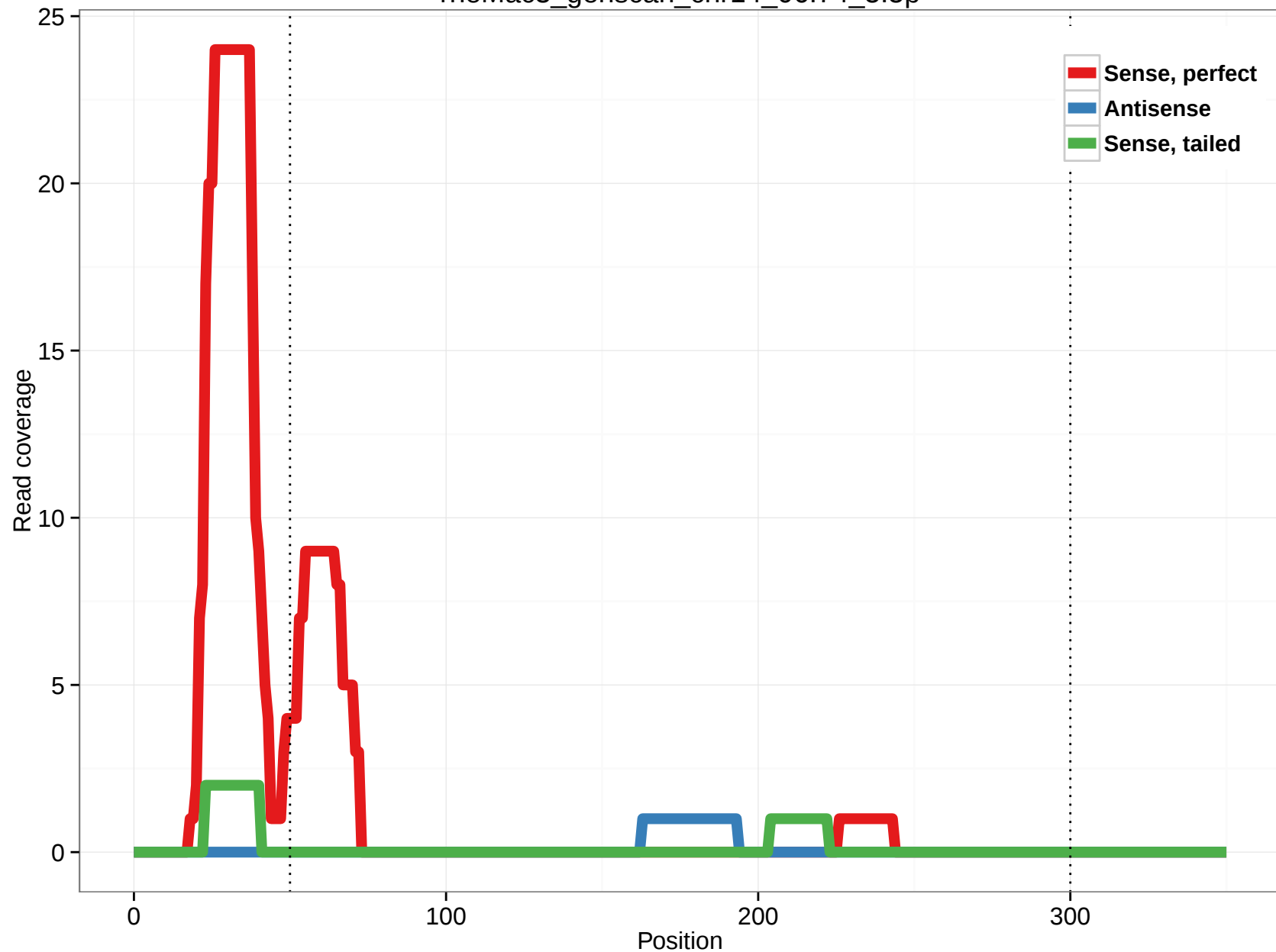
rheMac3_genscan_chr14_06.74_5.5p
