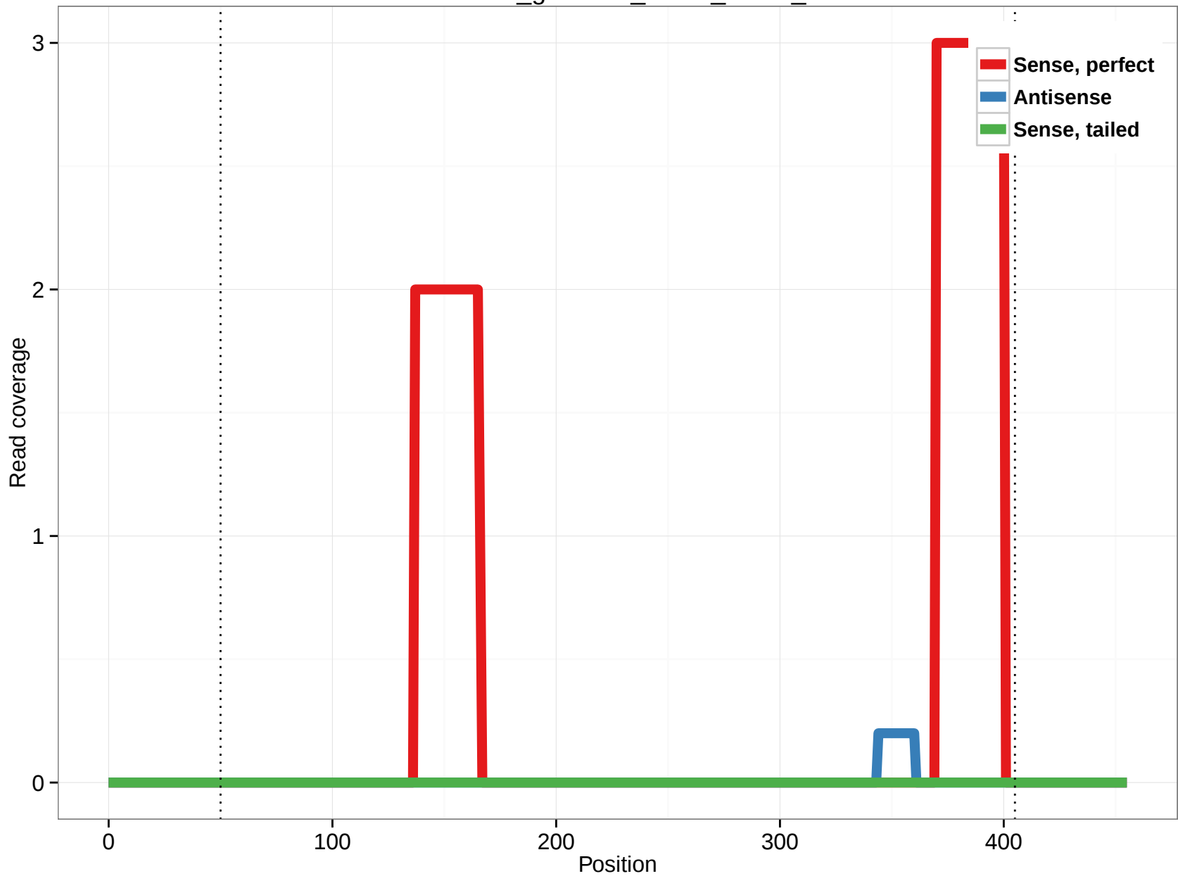
rheMac3_genscan_chr14_06.54_6
