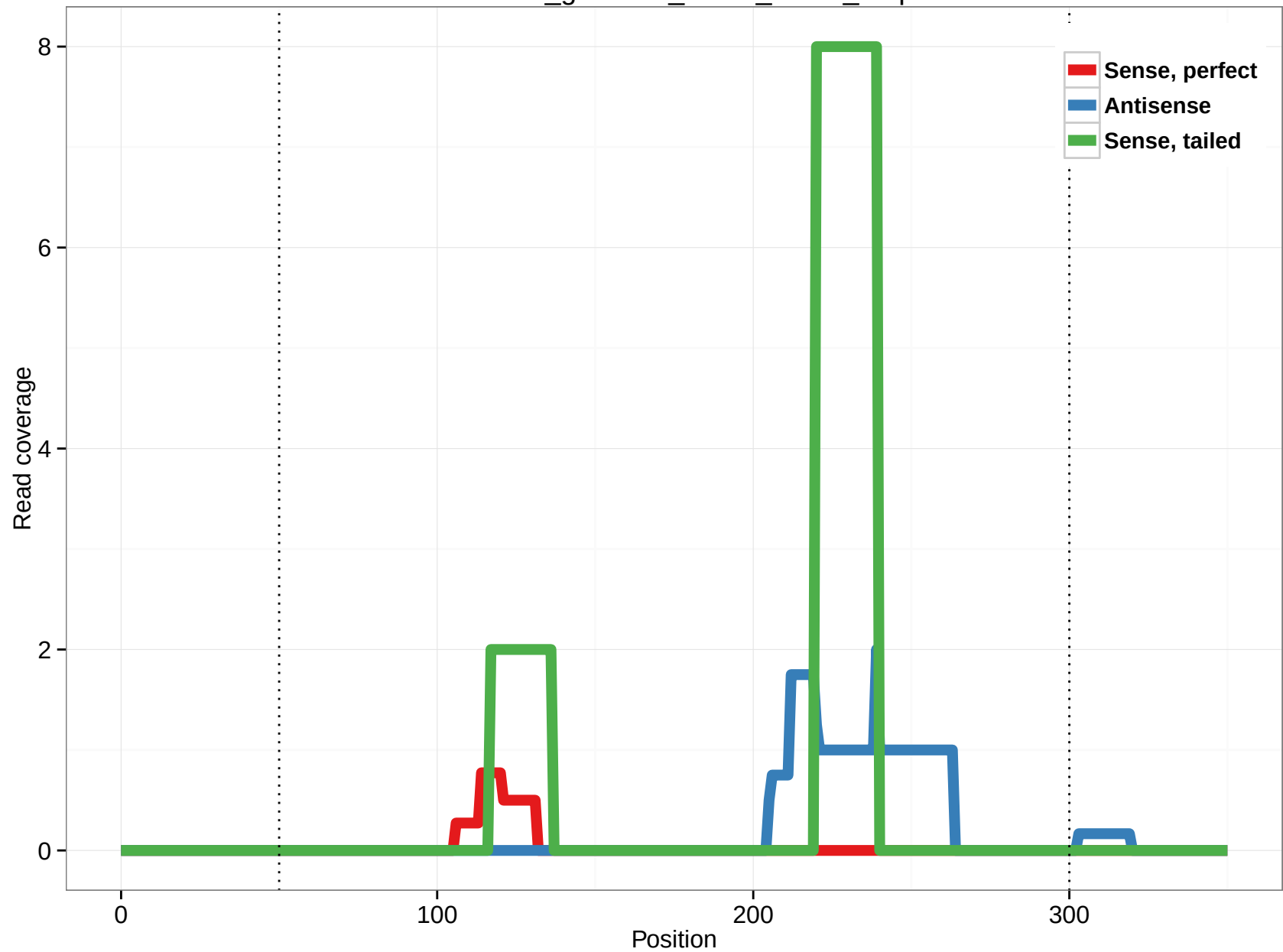
rheMac3_genscan_chr14_06.48_1.5p
