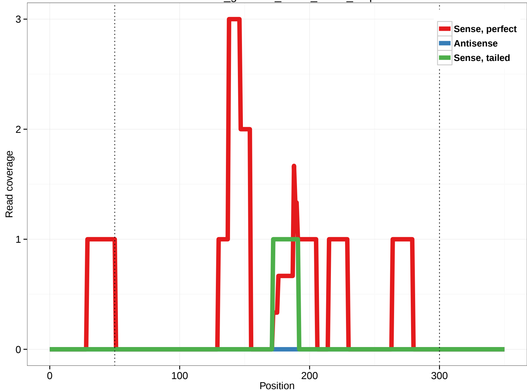
rheMac3_genscan_chr14_06.32_9.5p
