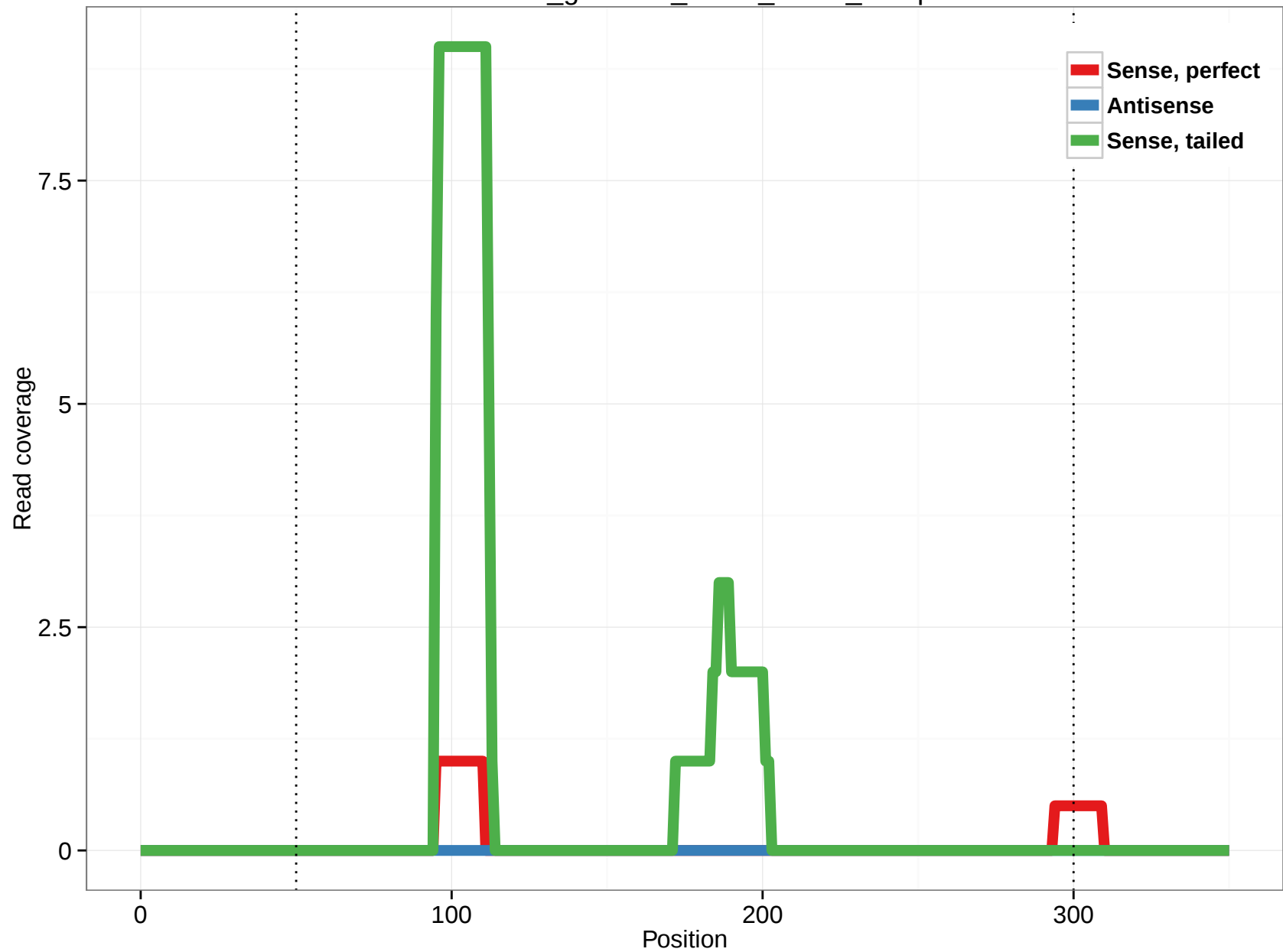
rheMac3_genscan_chr14_06.31_21.5p
