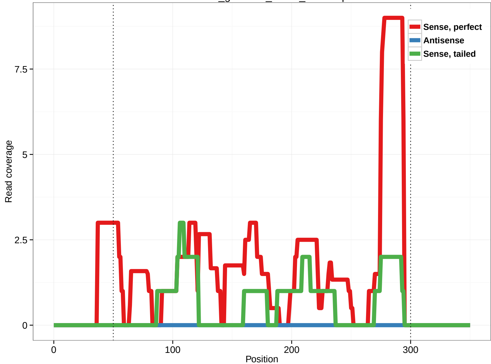
rheMac3_genscan_chr14_06.27.5p
