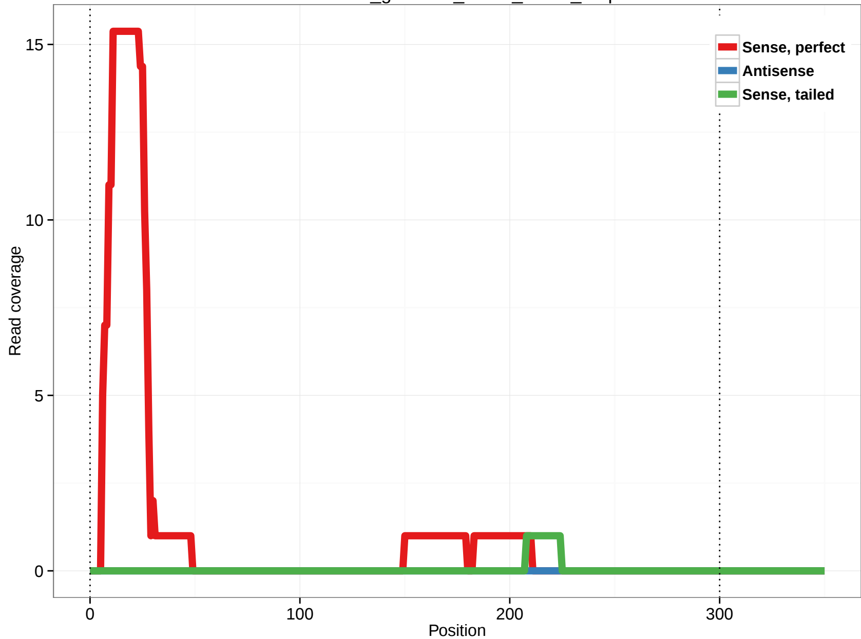
rheMac3_genscan_chr14_06.22_0.3p
