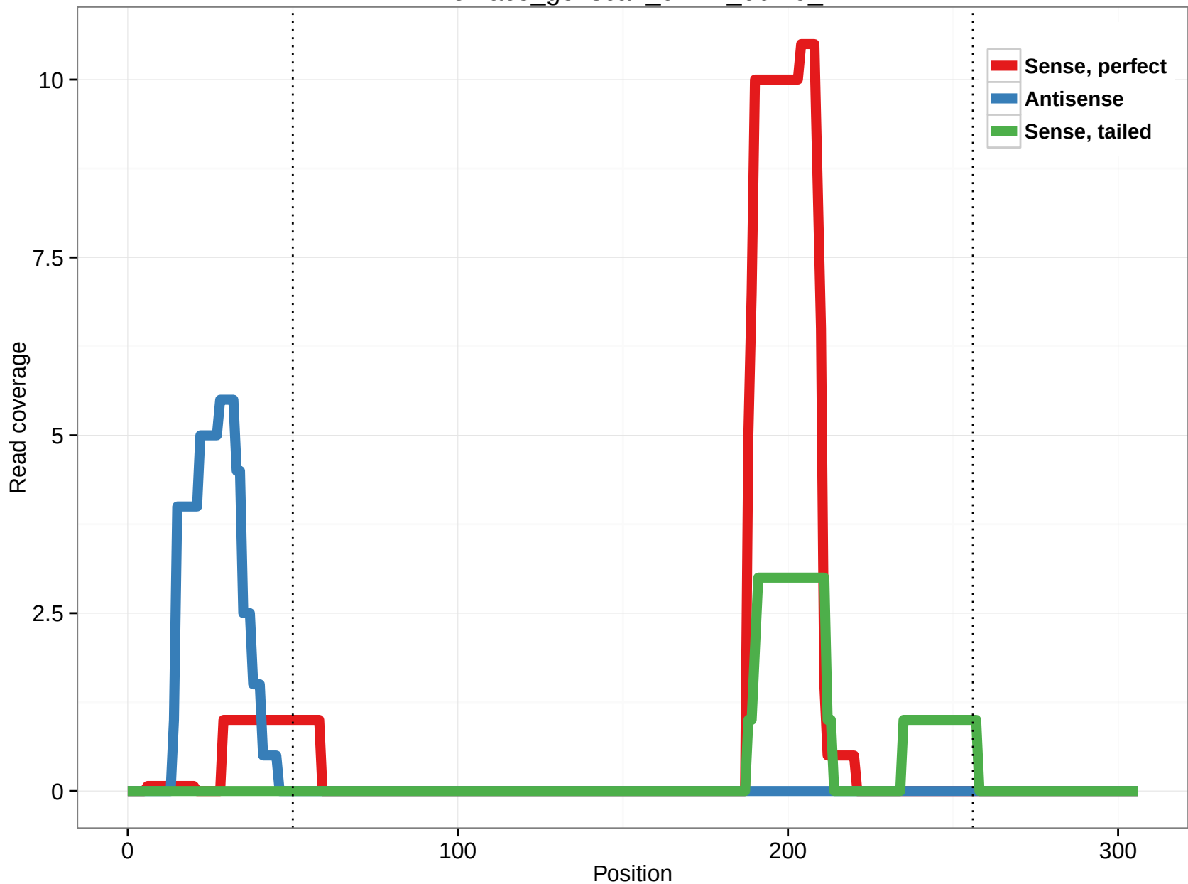
rheMac3_genscan_chr14_06.19_4
