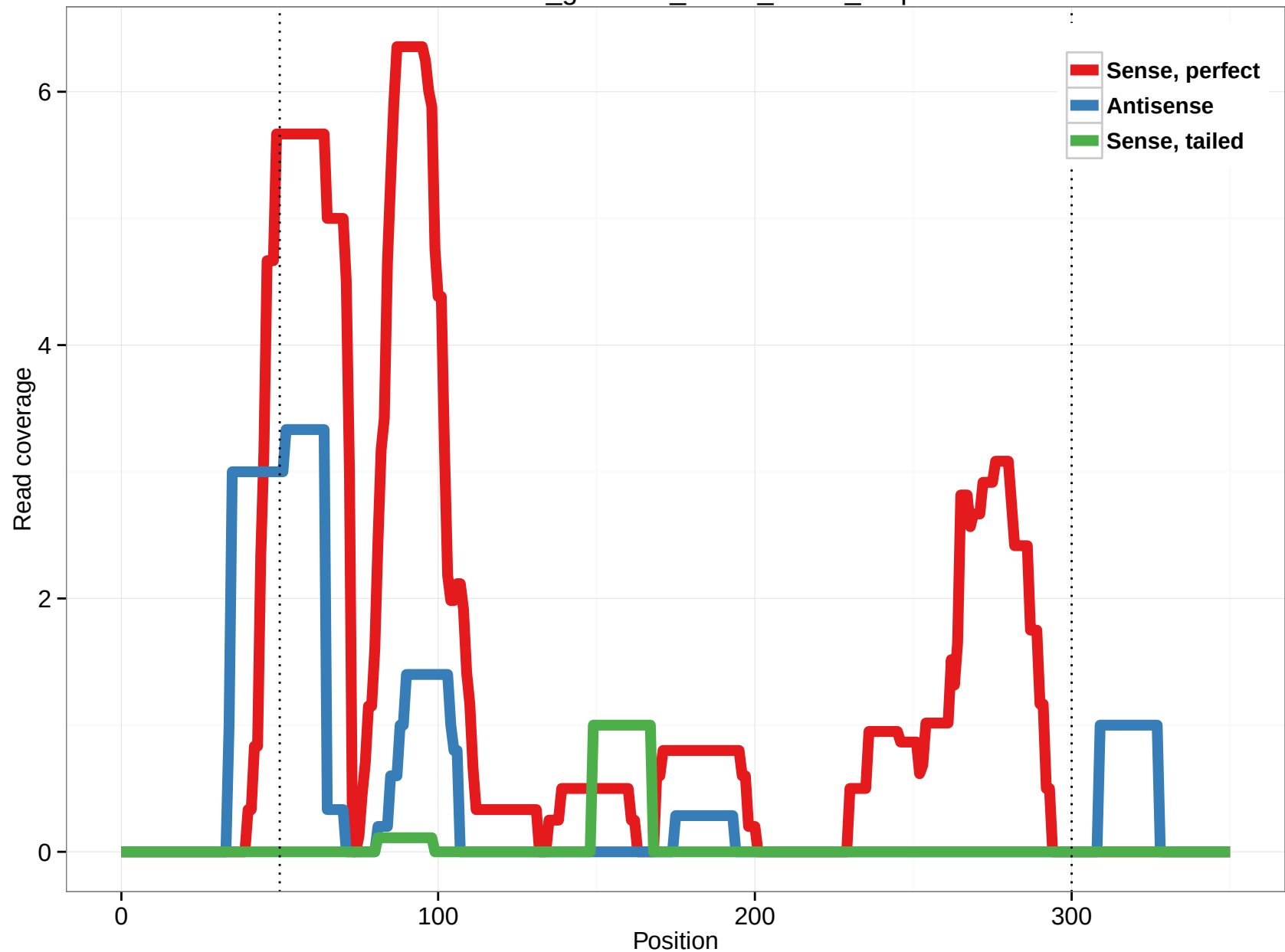
rheMac3_genscan_chr14_06.16_2.3p
