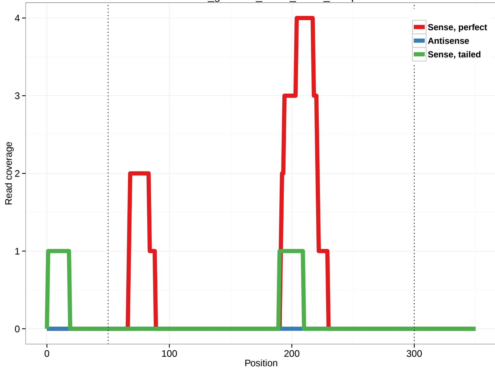
rheMac3_genscan_chr14_05.78_12.5p
