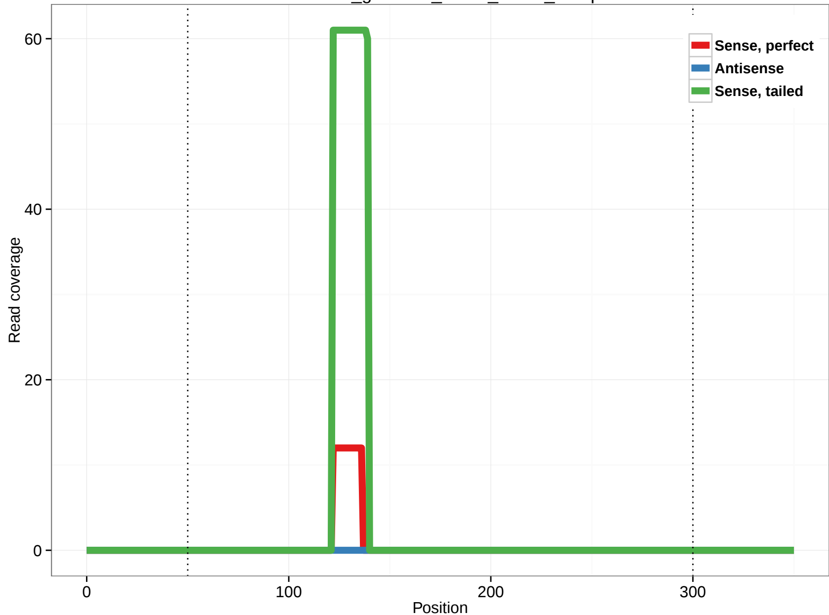
rheMac3_genscan_chr14_05.73_19.3p
