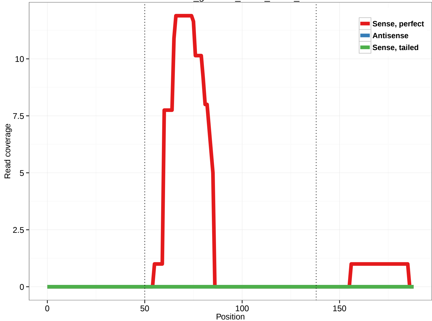
rheMac3_genscan_chr14_05.66_5
