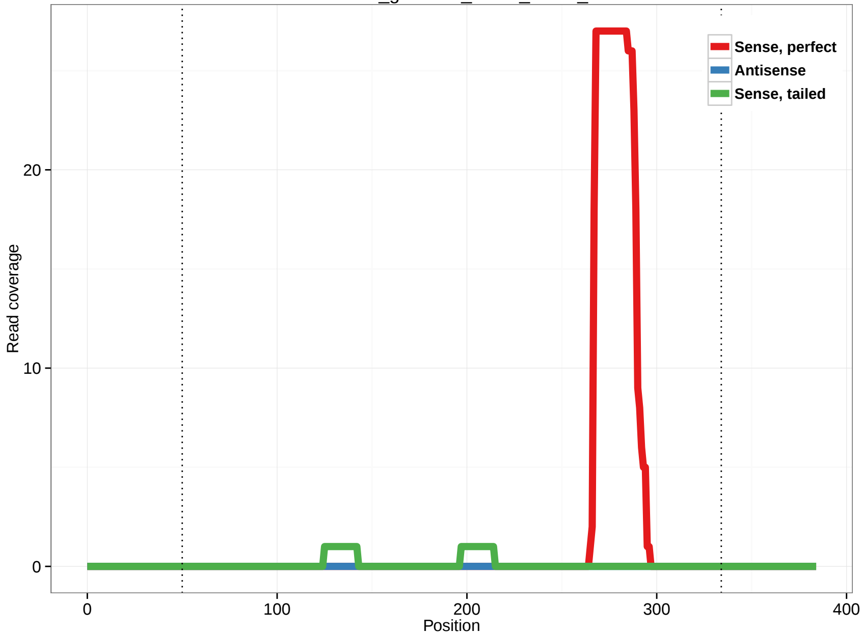
rheMac3_genscan_chr14_05.63_2
