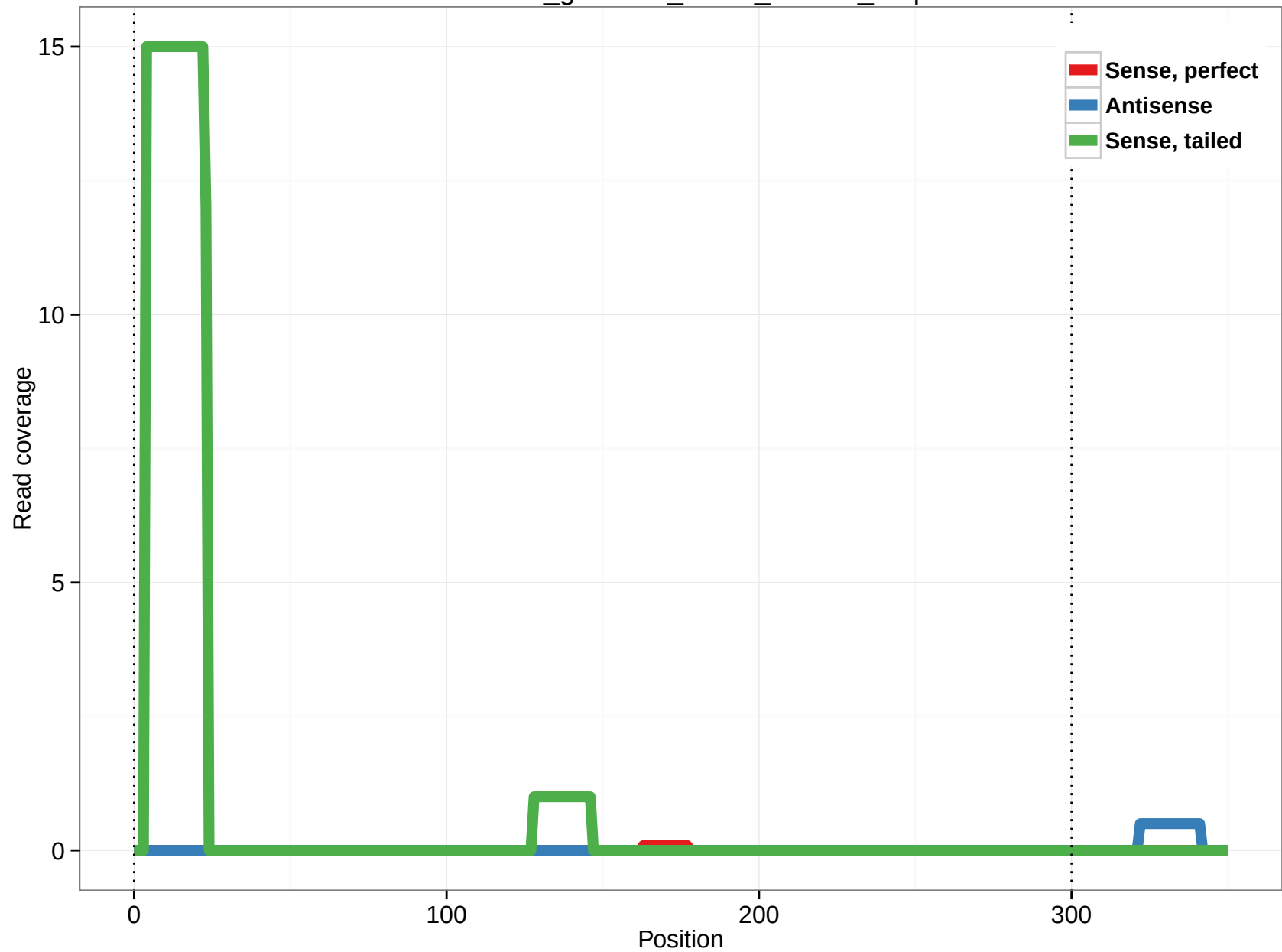
rheMac3_genscan_chr14_05.227_5.3p
