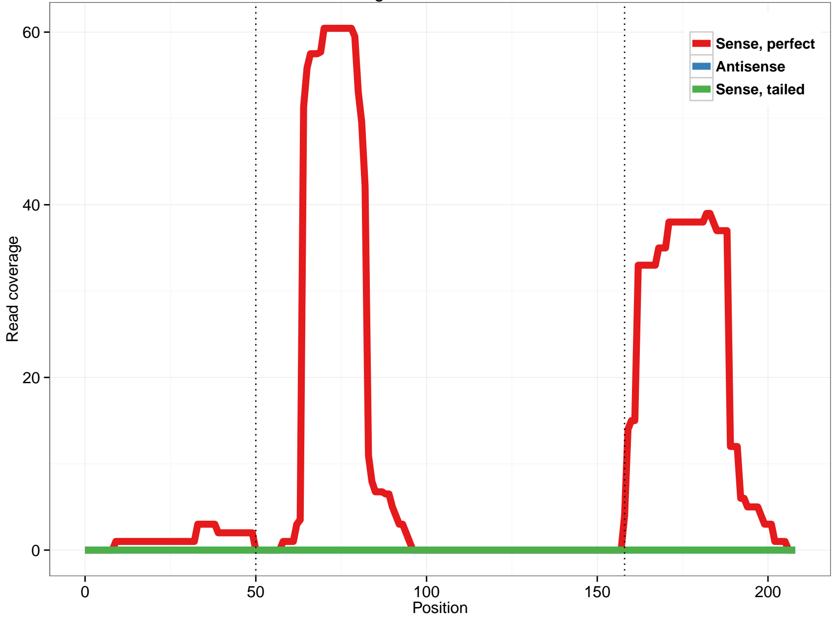
rheMac3_genscan_chr14_05.225_4
