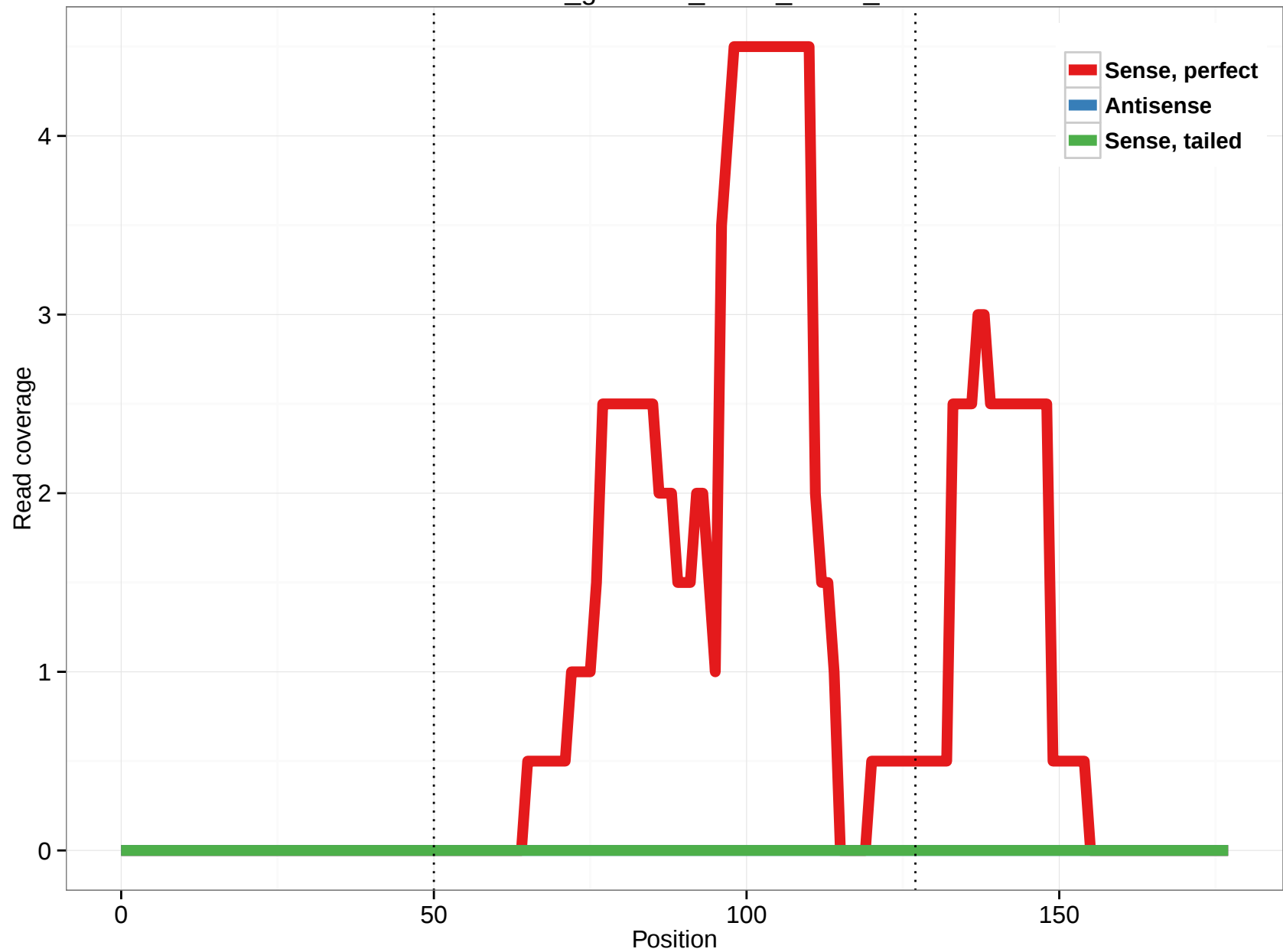
rheMac3_genscan_chr14_05.21_0
