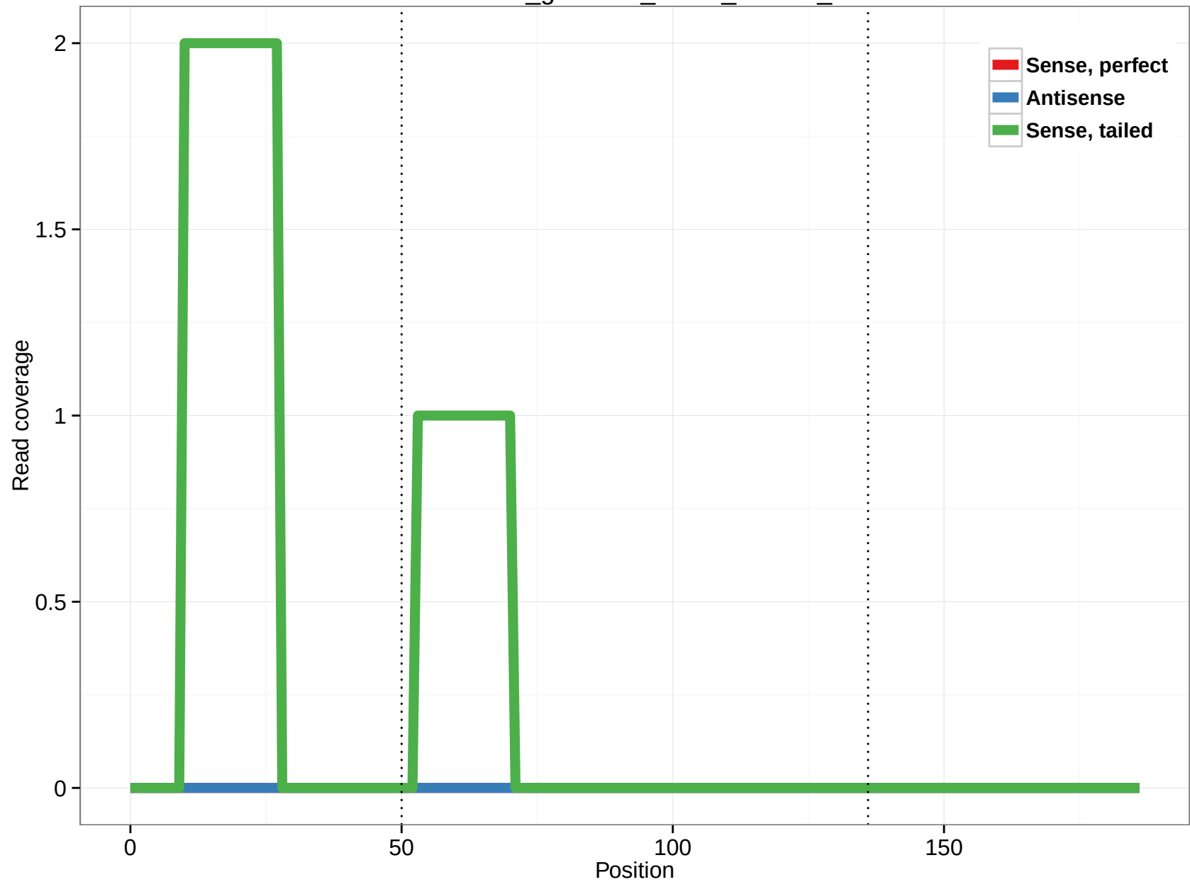
rheMac3_genscan_chr14_05.213_1
