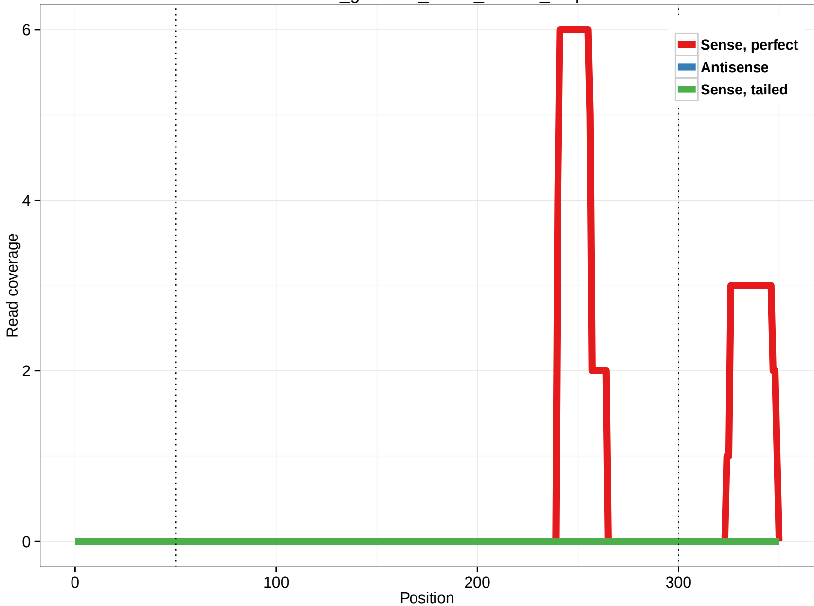
rheMac3_genscan_chr14_05.209_4.3p
