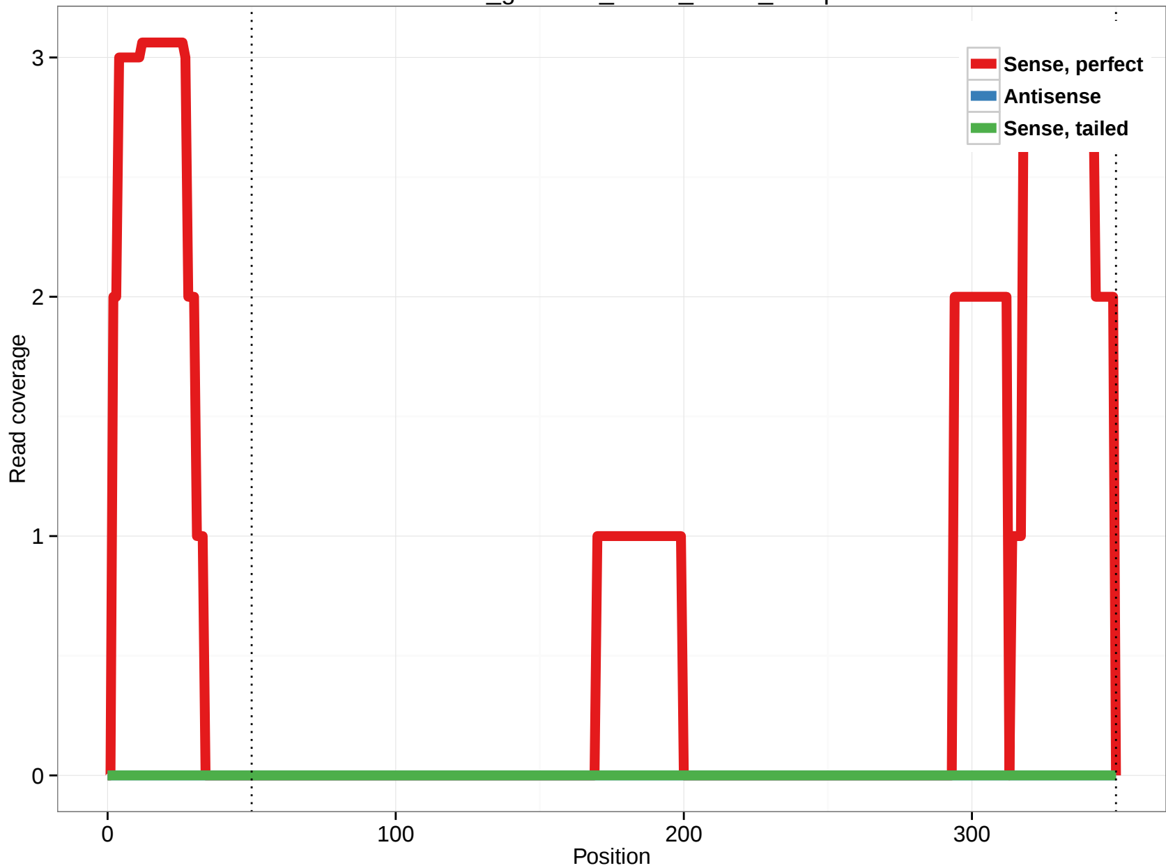
rheMac3_genscan_chr14_05.18_25.5p
