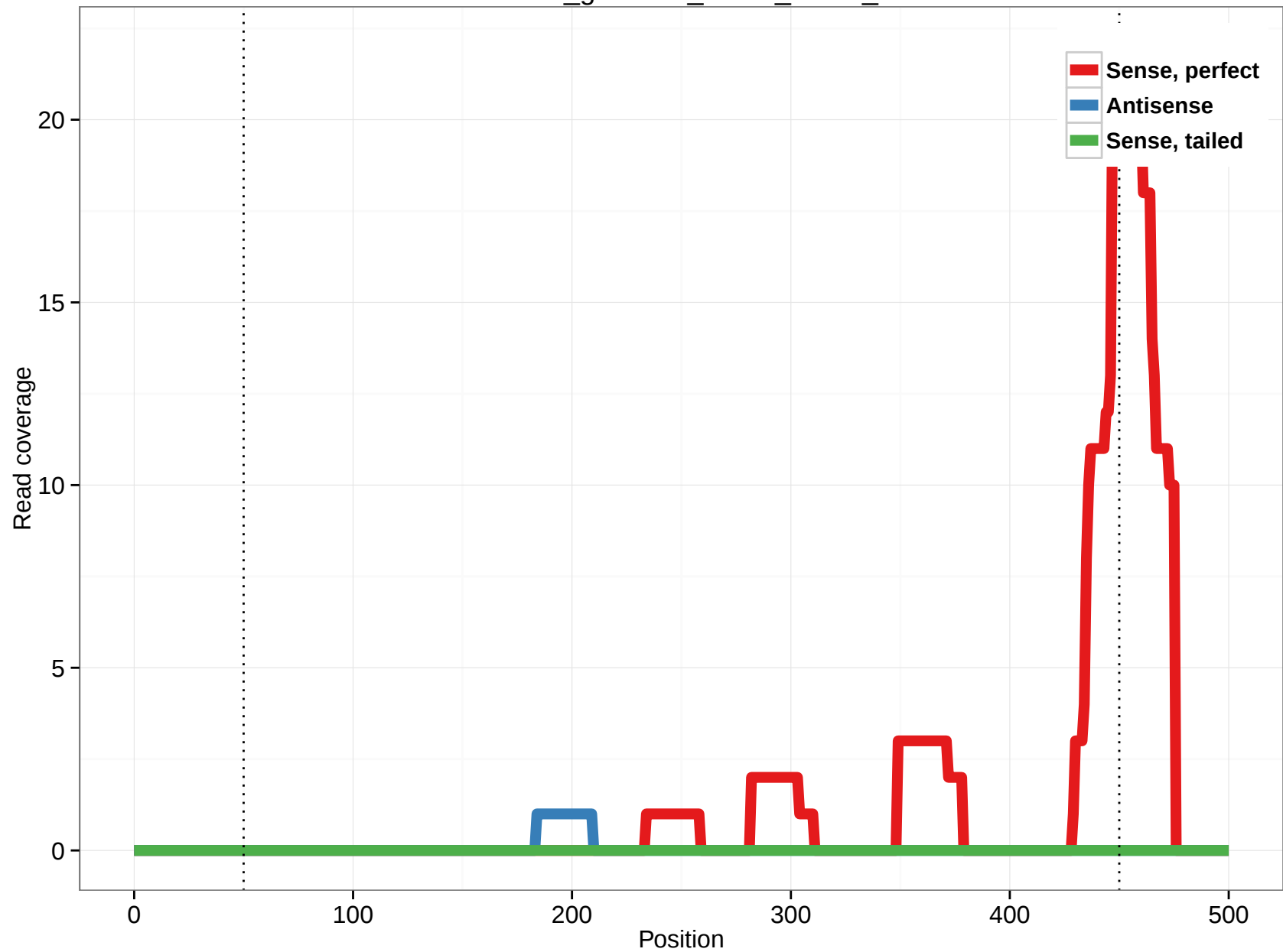
rheMac3_genscan_chr14_05.16_22
