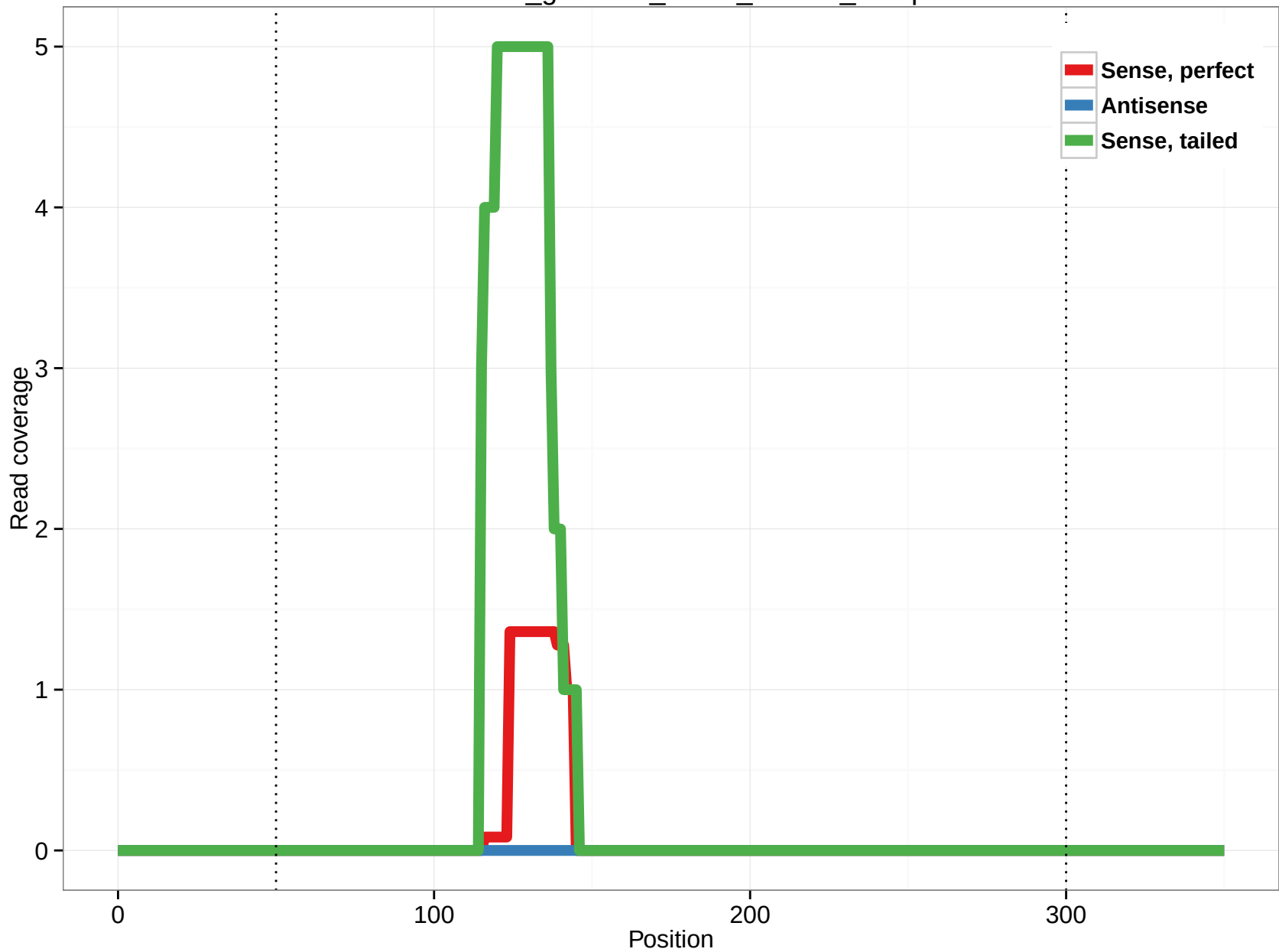
rheMac3_genscan_chr14_05.153_16.3p
