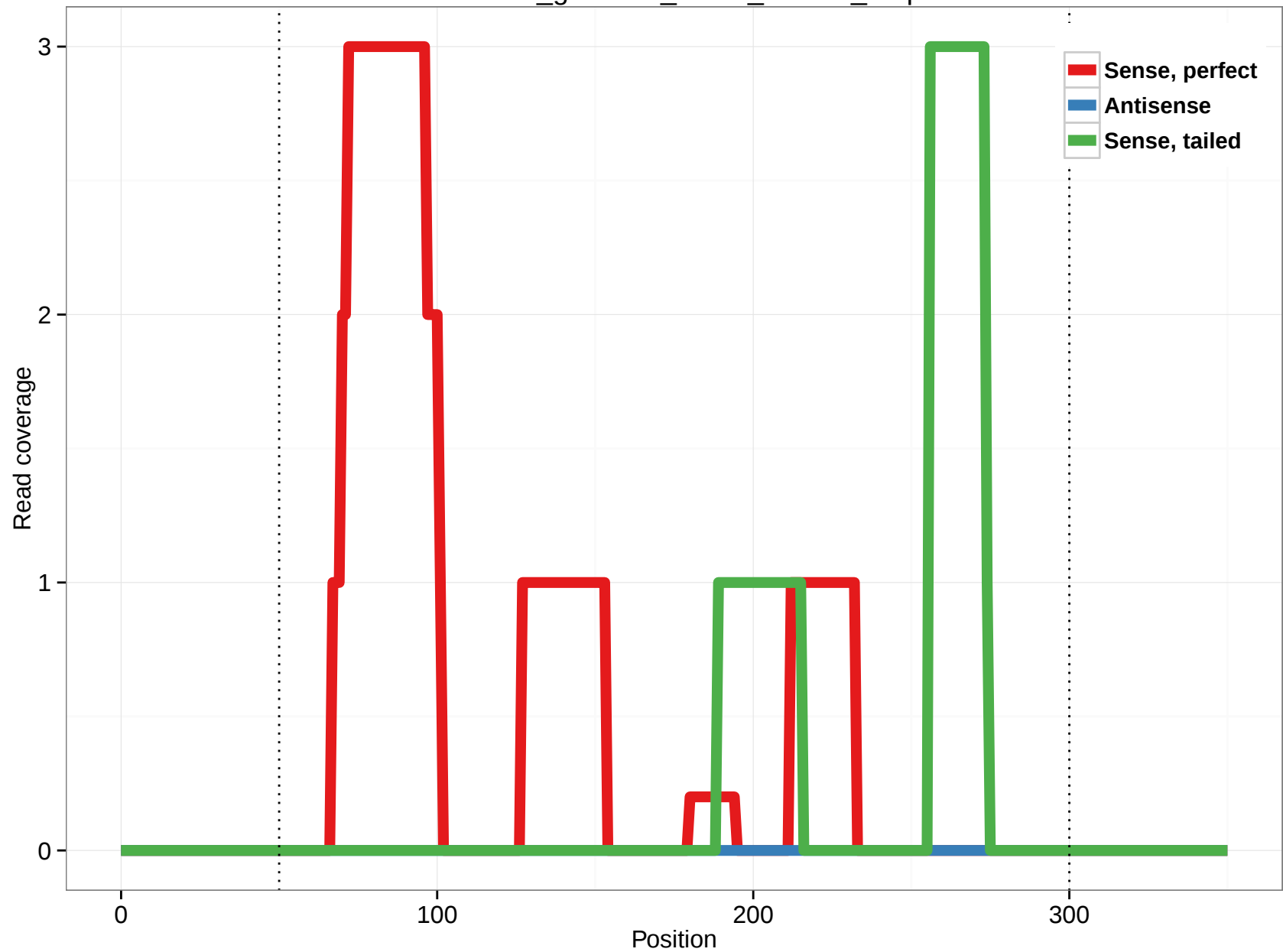
rheMac3_genscan_chr14_05.134_0.5p
