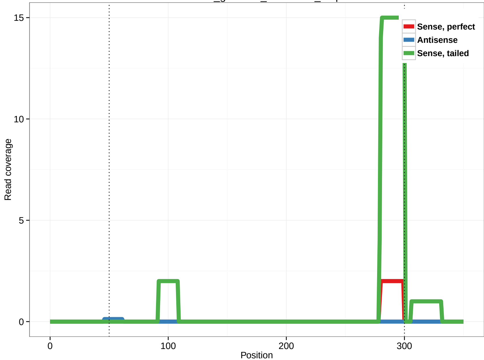
rheMac3_genscan_chr14.119_6.3p
