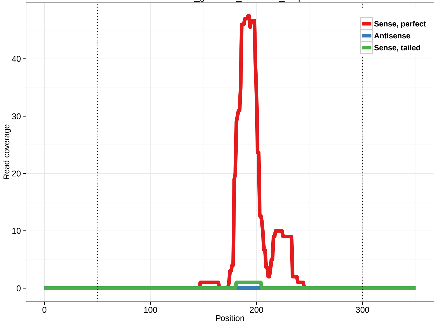
rheMac3_genscan_chr14.07_7.3p
