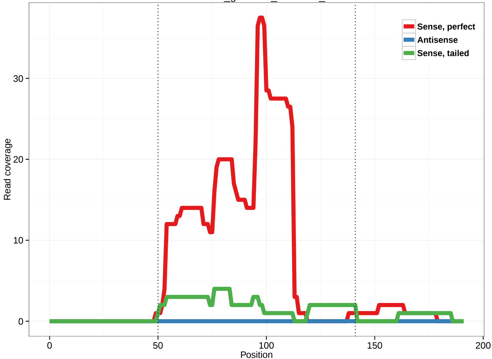
rheMac3_genscan_chr14.02_6
