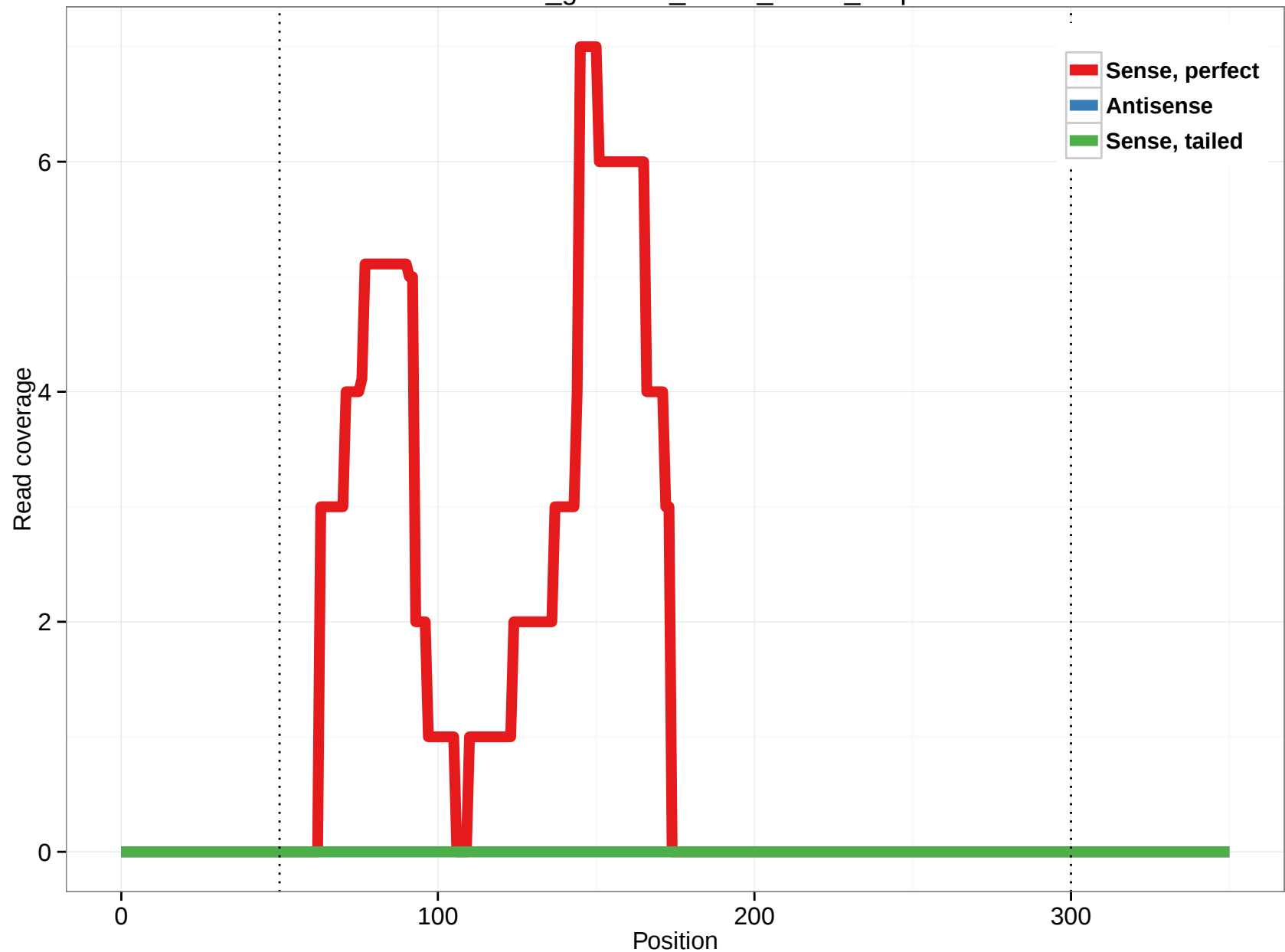
rheMac3_genscan_chr13_85.22_3.5p
