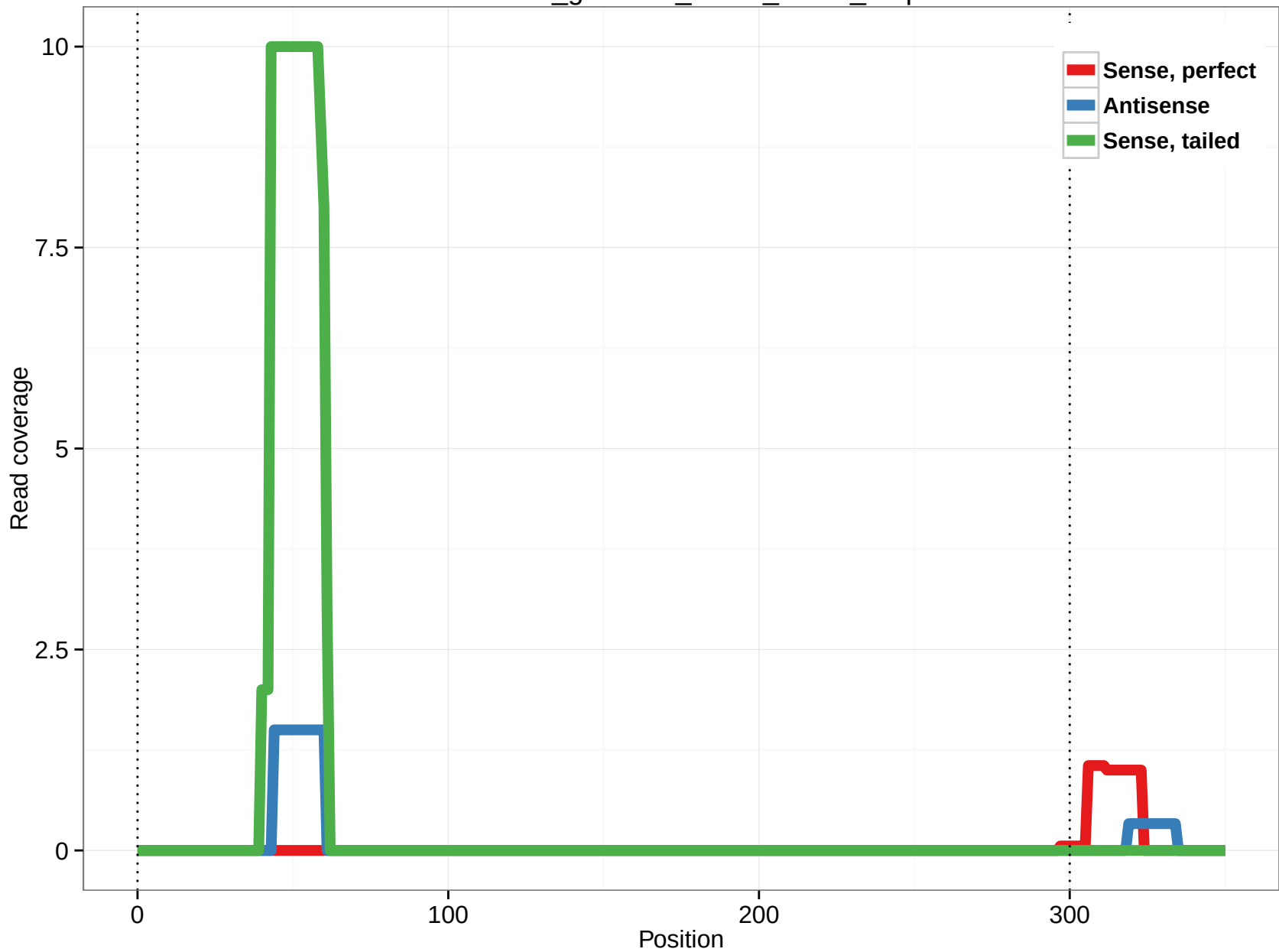
rheMac3_genscan_chr13_85.19_8.3p
