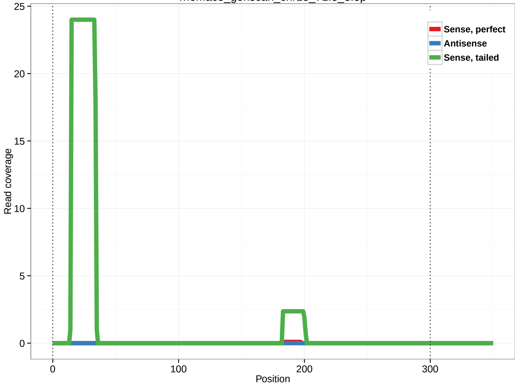
rheMac3_genscan_chr13_71.3_3.3p
