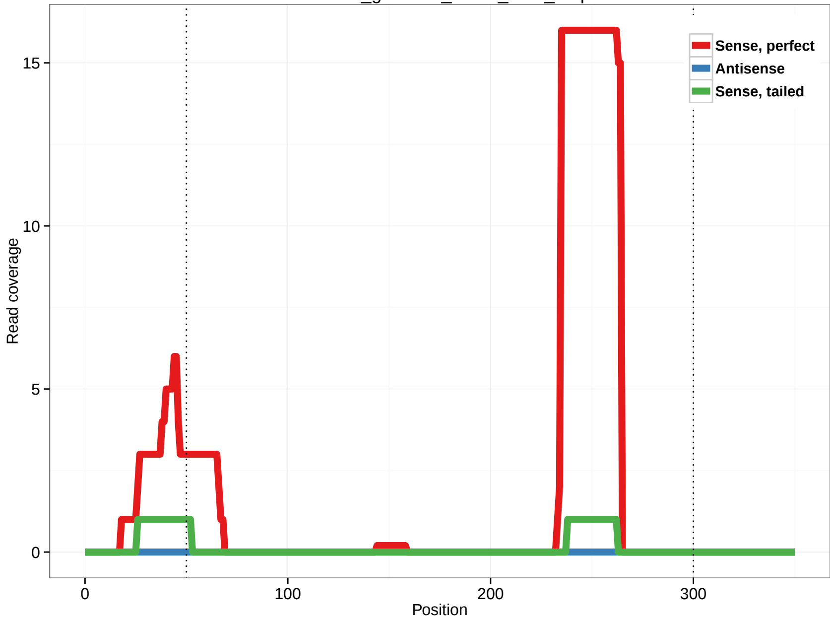
rheMac3_genscan_chr13_58.5_1.5p
