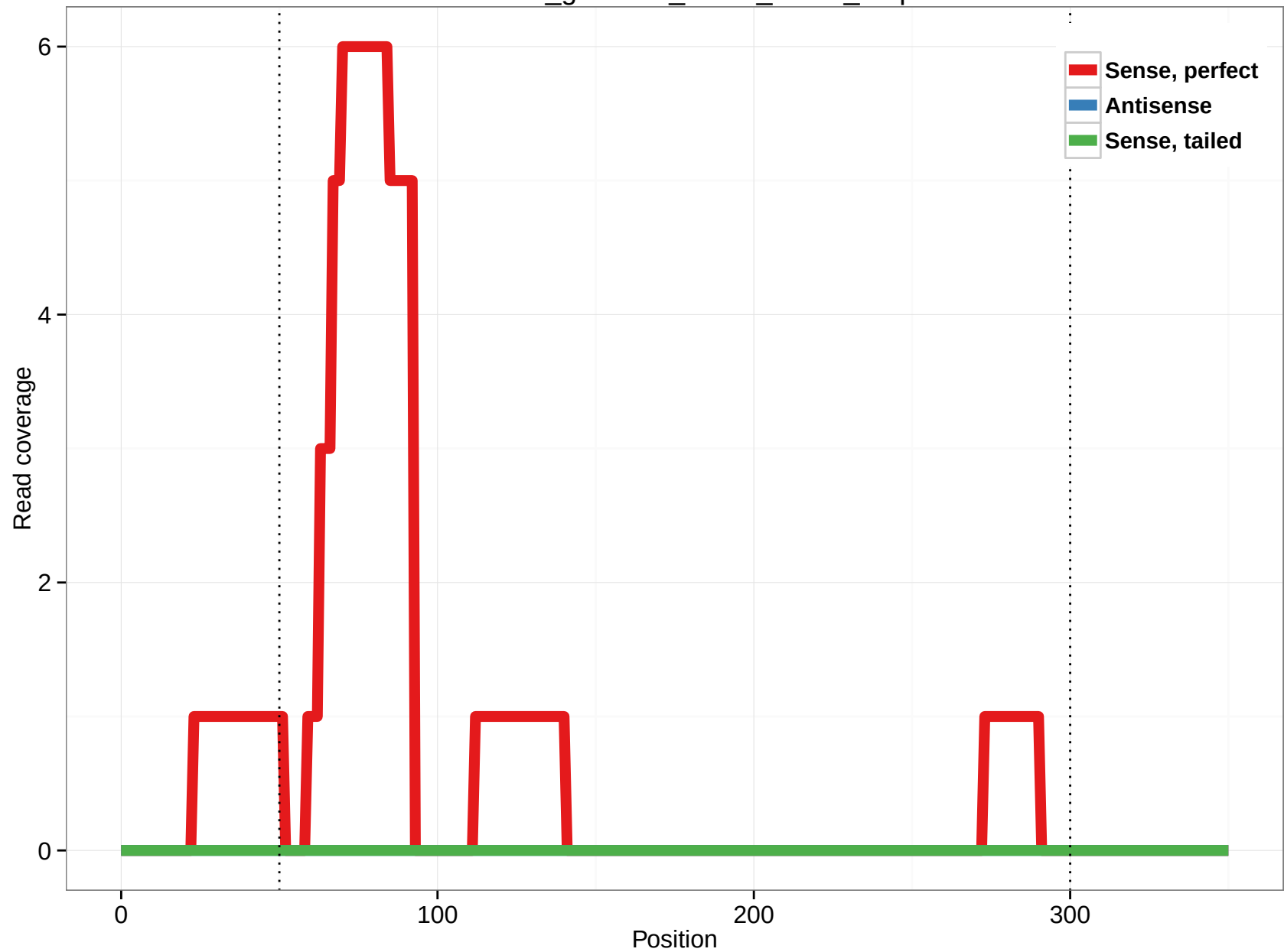
rheMac3_genscan_chr13_58.48_6.3p
