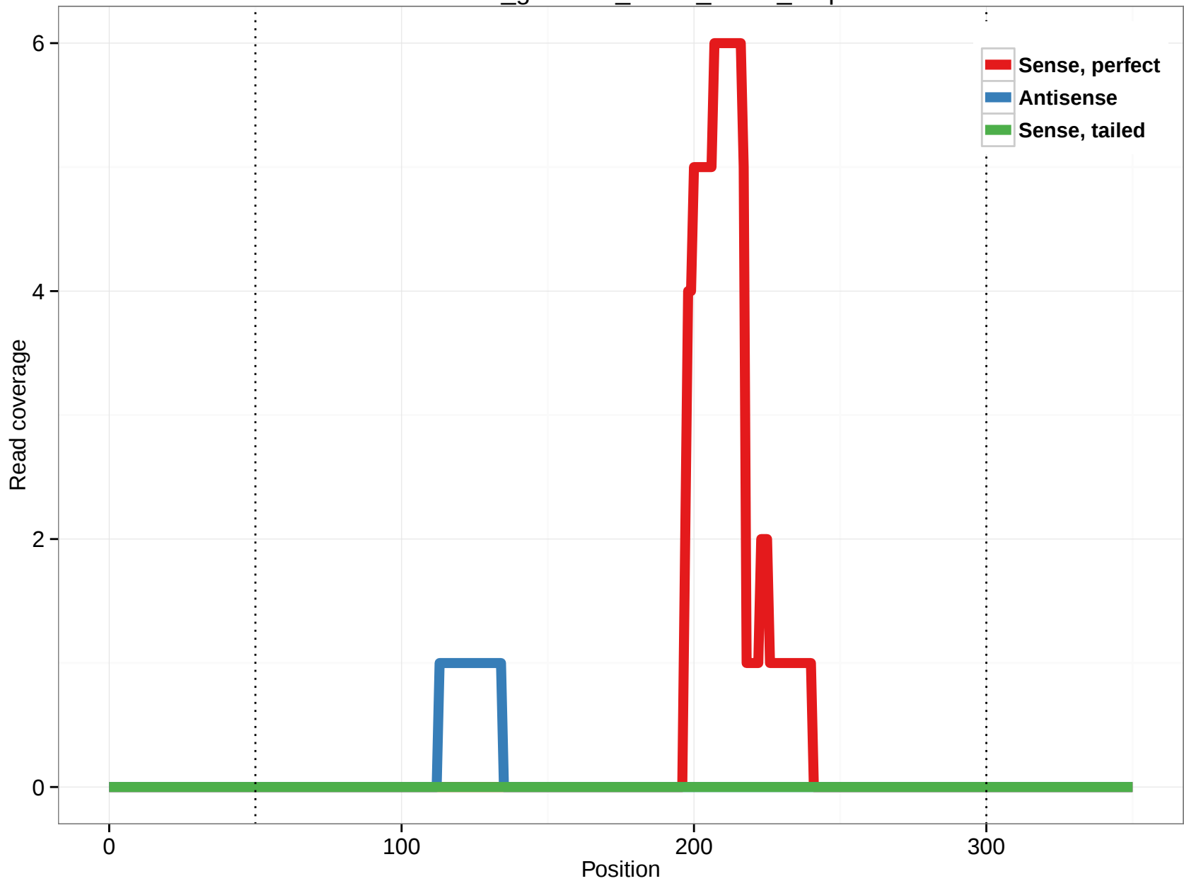
rheMac3_genscan_chr13_58.25_0.5p
