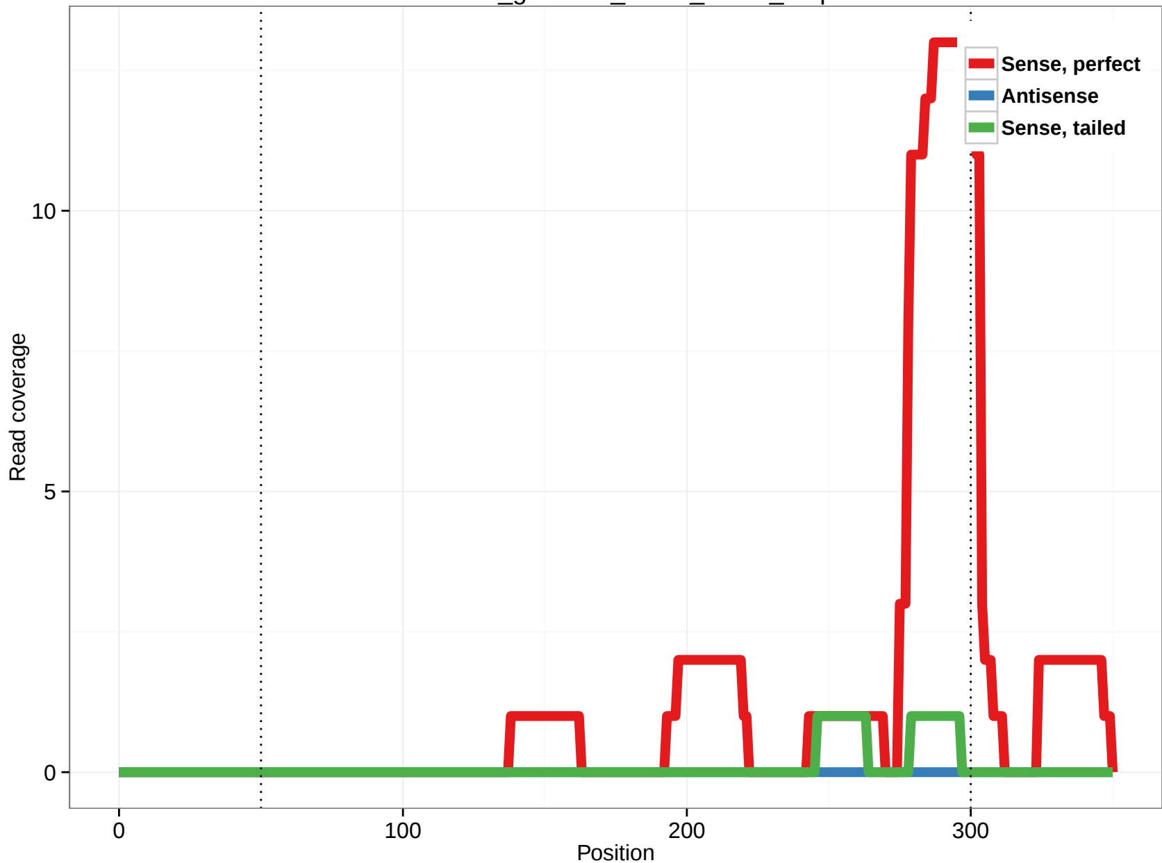
rheMac3_genscan_chr13_58.23_6.3p
