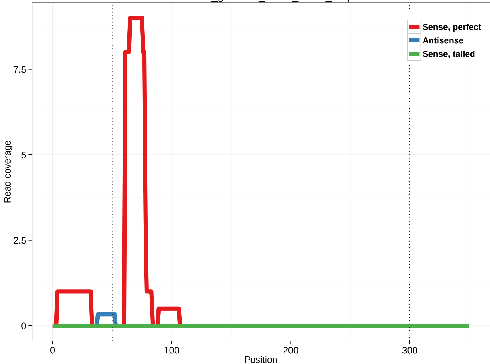
rheMac3_genscan_chr13_55.63_6.5p
