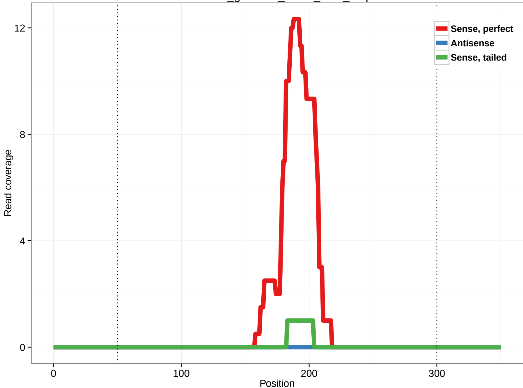
rheMac3_genscan_chr13_52.4_5.3p
