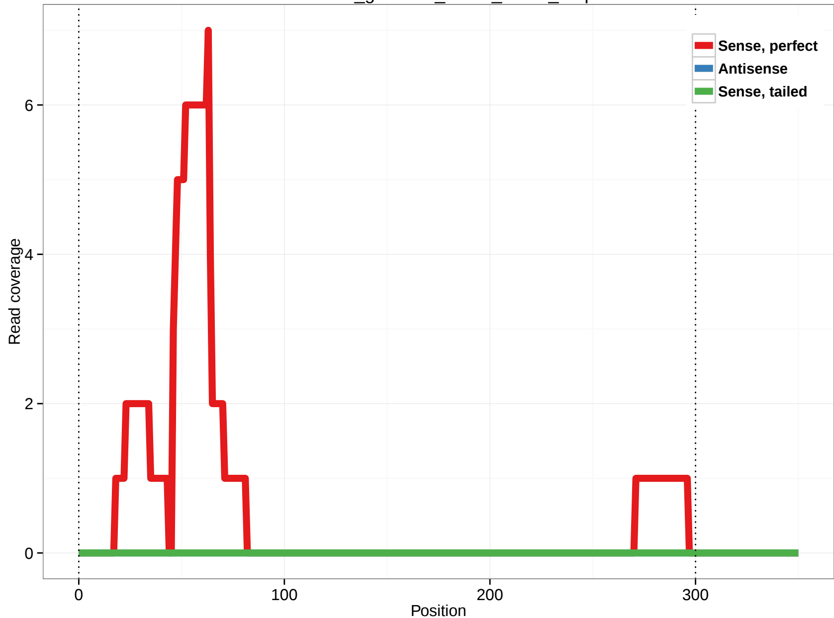
rheMac3_genscan_chr13_51.22_1.3p
