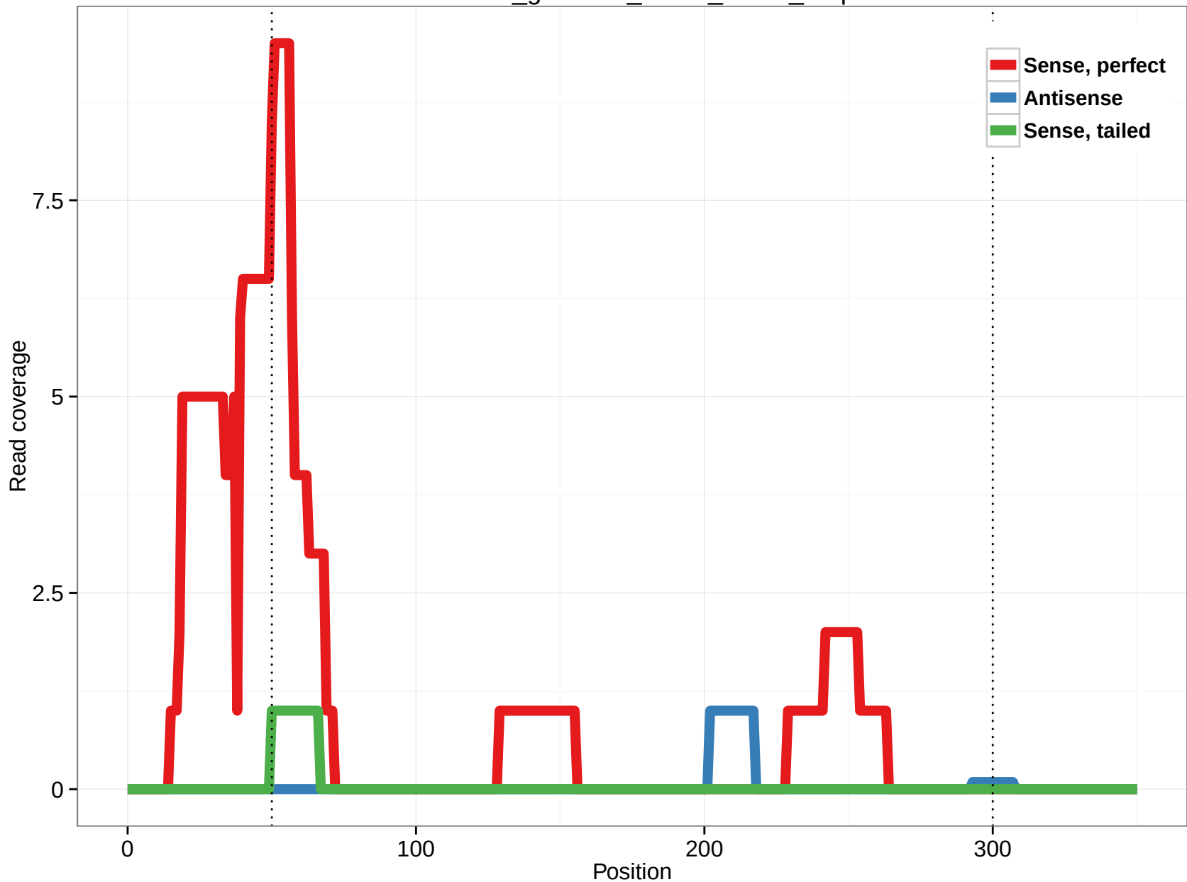
rheMac3_genscan_chr13_47.19_1.5p
