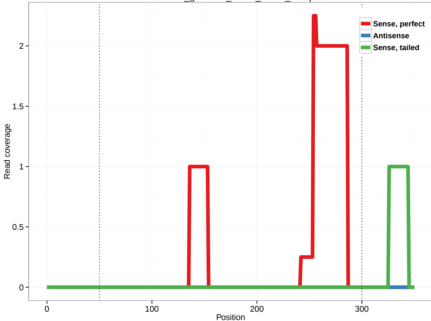
rheMac3_genscan_chr13_47.12_34.3p
