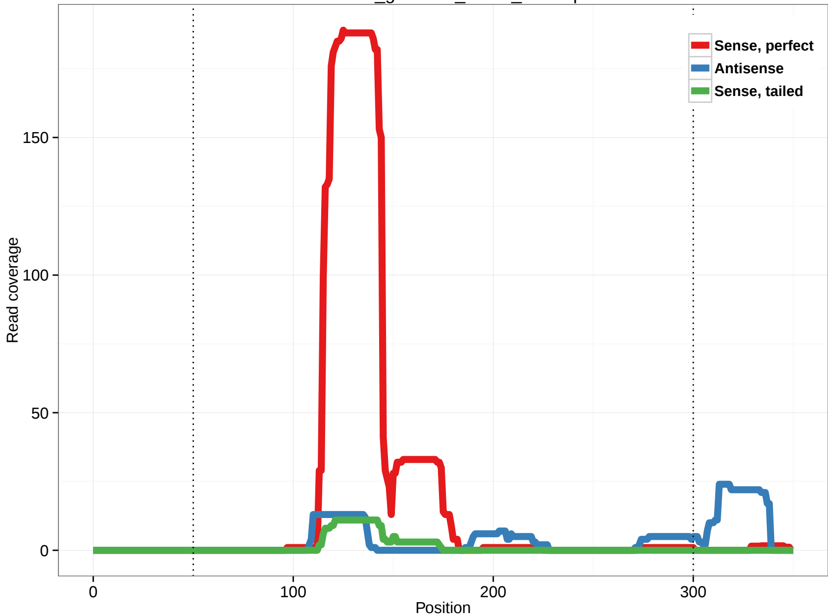
rheMac3_genscan_chr13_43.2.3p
