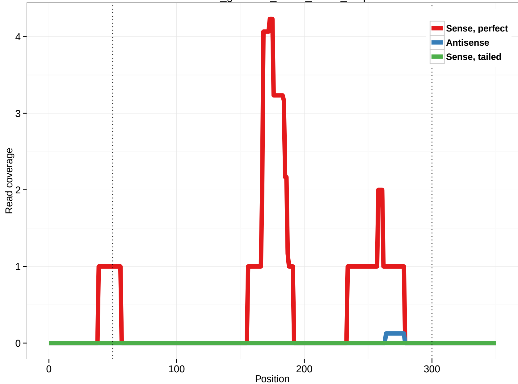
rheMac3_genscan_chr13_32.57_7.5p
